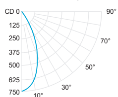
Wide flood 44° (3000K, 90CRI)
